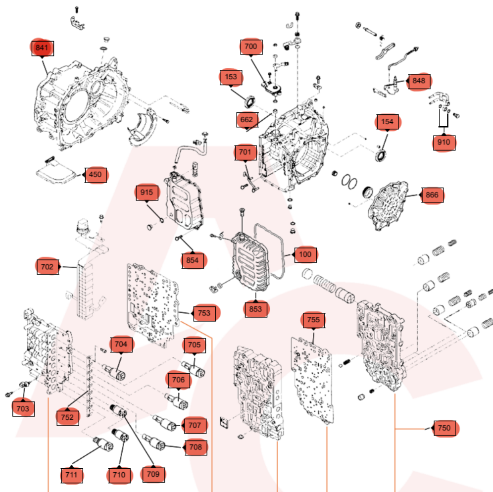
Casing and Valve Body Components
